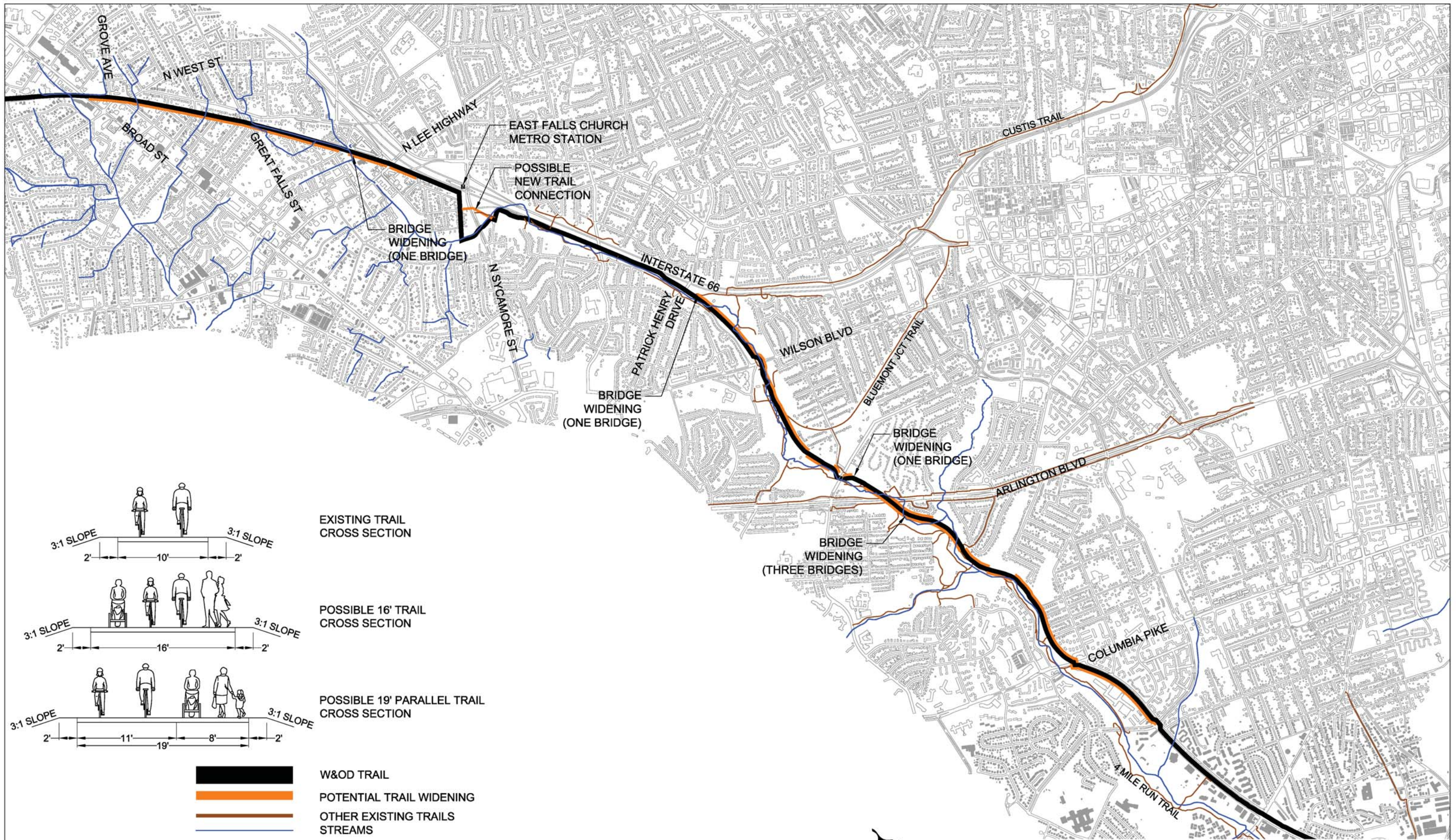
FIGURE 2. TRAIL WIDENING FEASIBILITY AND CONSTRAINTS W&OD PARALLEL TRAIL STUDY
